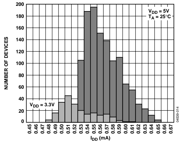
Figure 20. I_{DD} Histogram
